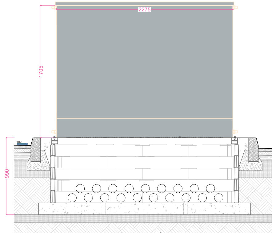
Rear Sectional Elevation
