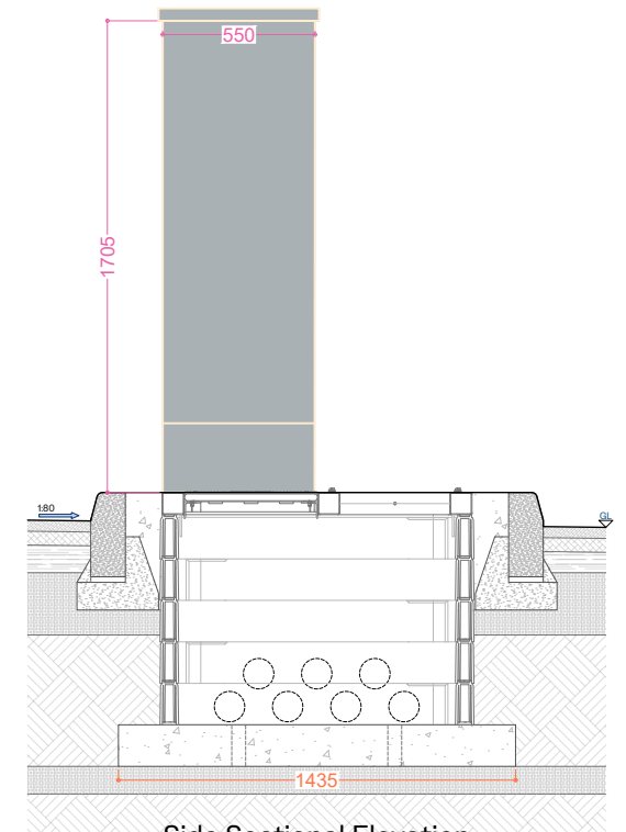
Side Sectional Elevation
