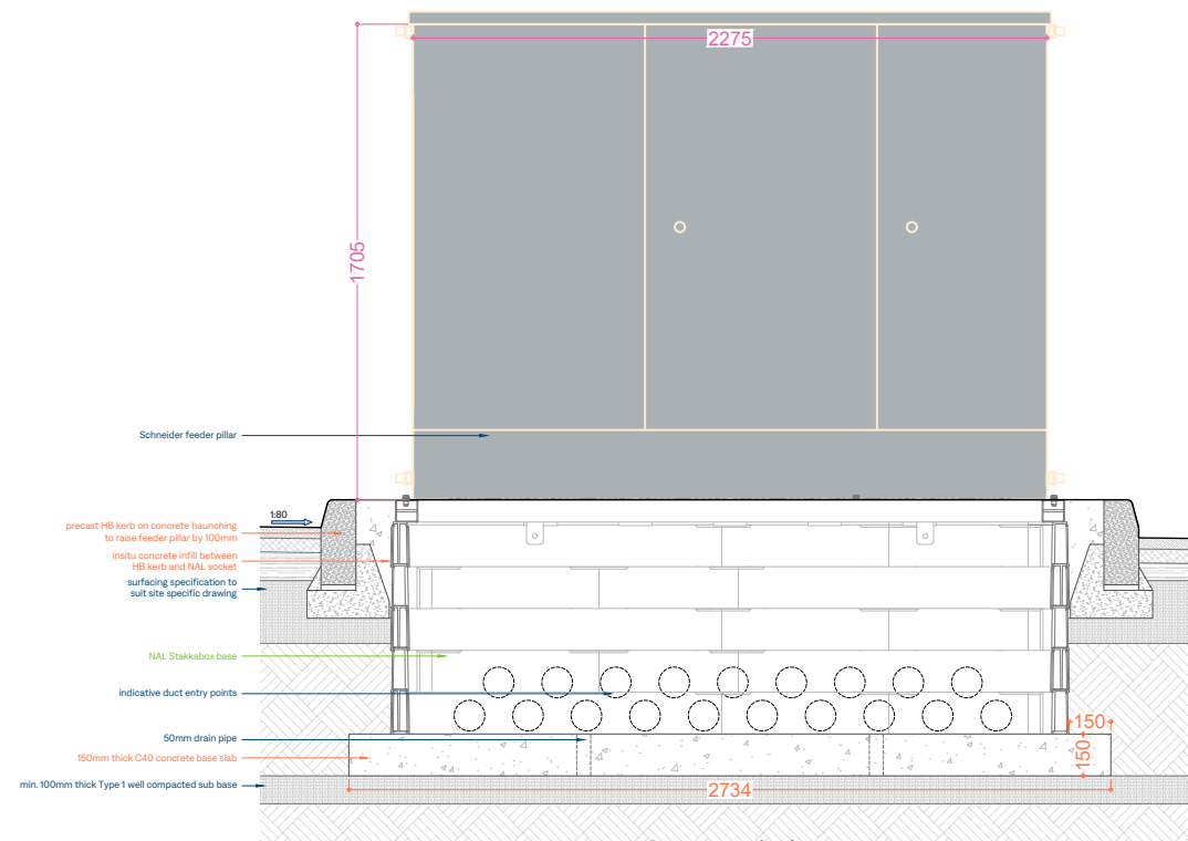
Front Sectional Elevation
