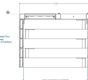
Section BB feeder pillar omitted for clarity
