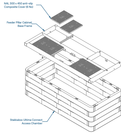
Exploded view feeder pillar omitted for clarity
