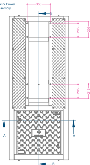
Plan Elevatio
