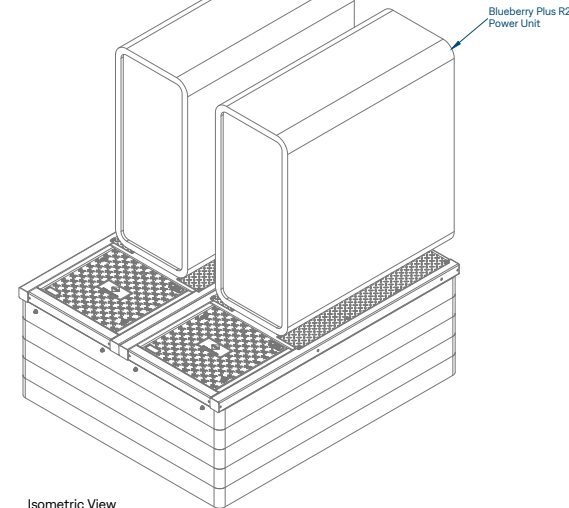
Isometric View Two Power Units Base
