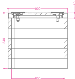
Section A
