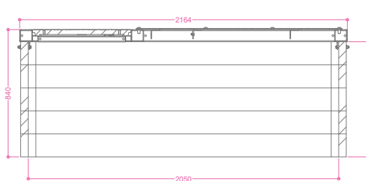
Section B
