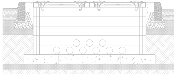
Side Sectional Elevation
