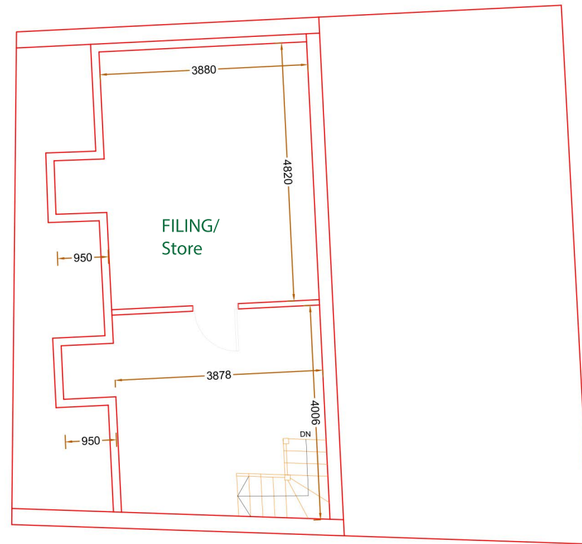
EXISTING LOFT FLOOR PLAN
