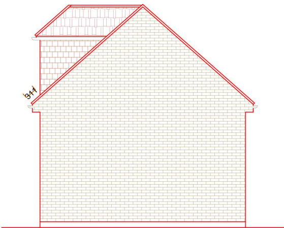
PROPOSED SIDE ELEVATION-1 50(A) MOUNT PLEASANT
