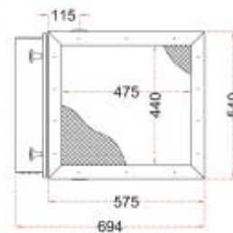
End View Air Inlet
