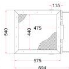
End View
