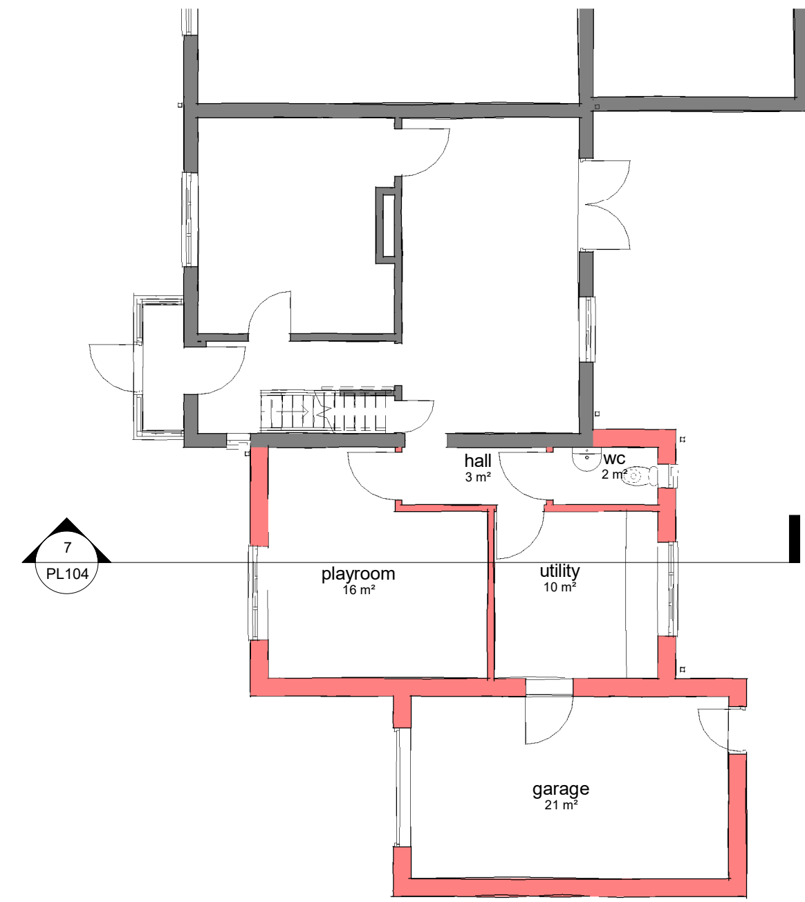
2 Ground Floor 1 : 100
