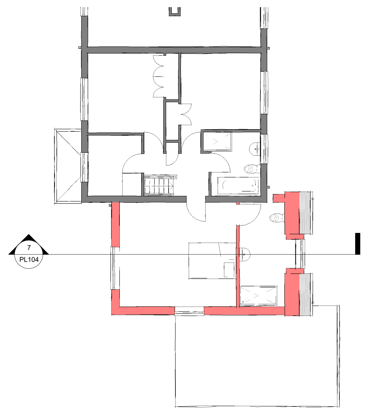
3 First Floor 1 : 100
