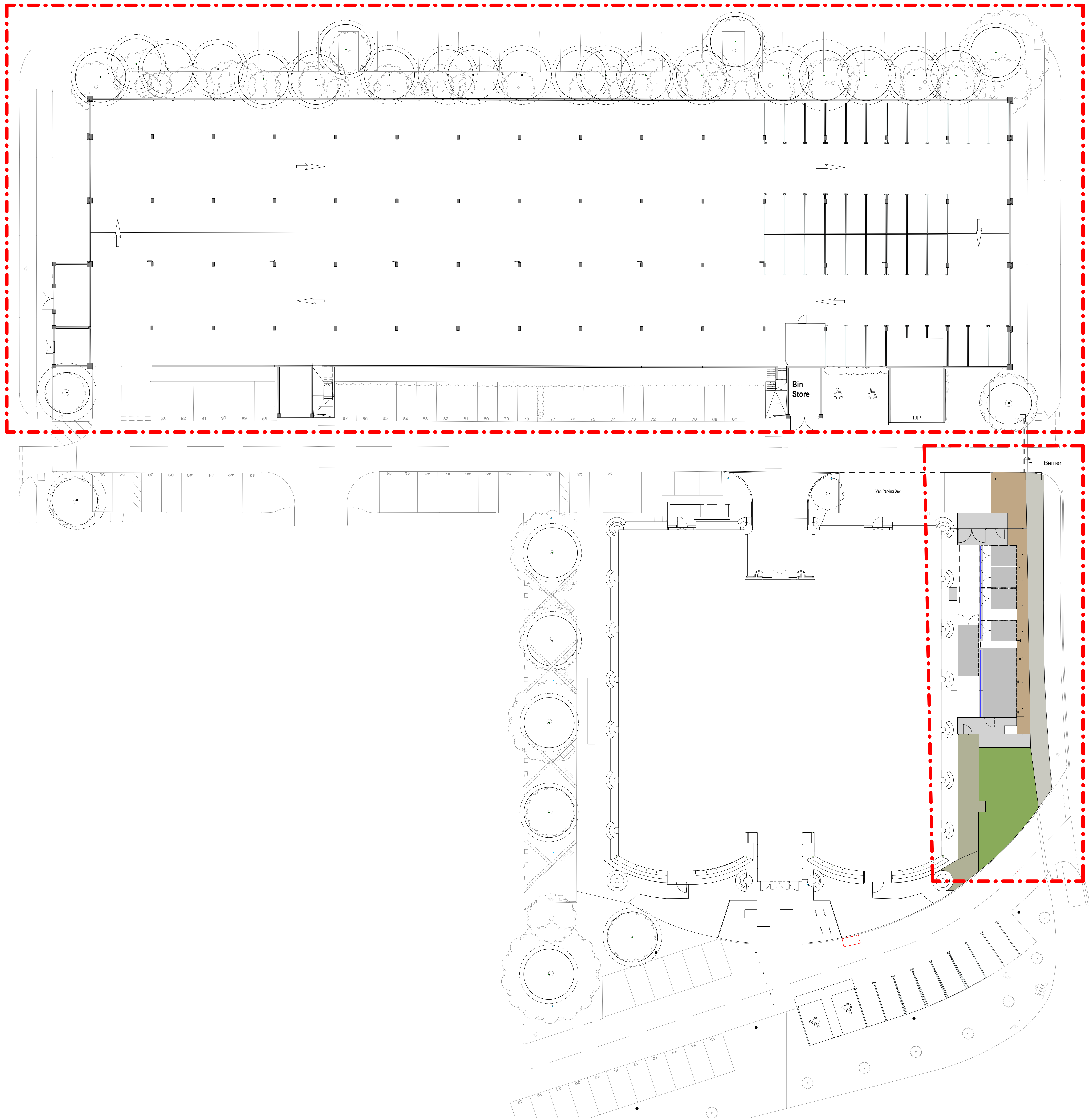
1 Site Arrangement Plan 1:200
