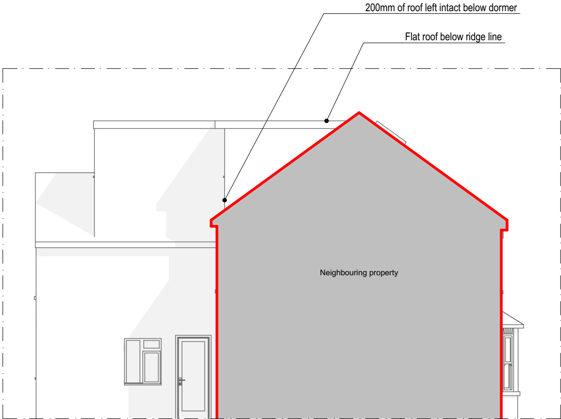
E-04 Left Side Elevation (1) 1:100
