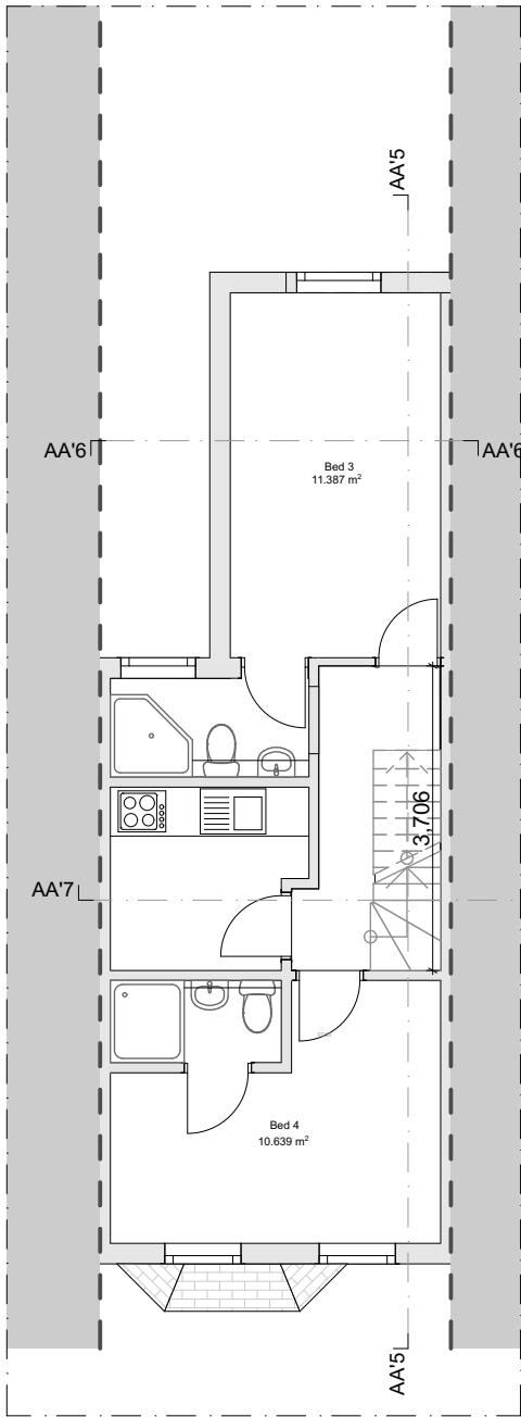
1. First Floor (1) 1:100
