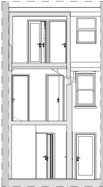
AA'6 Building Section 1:100
