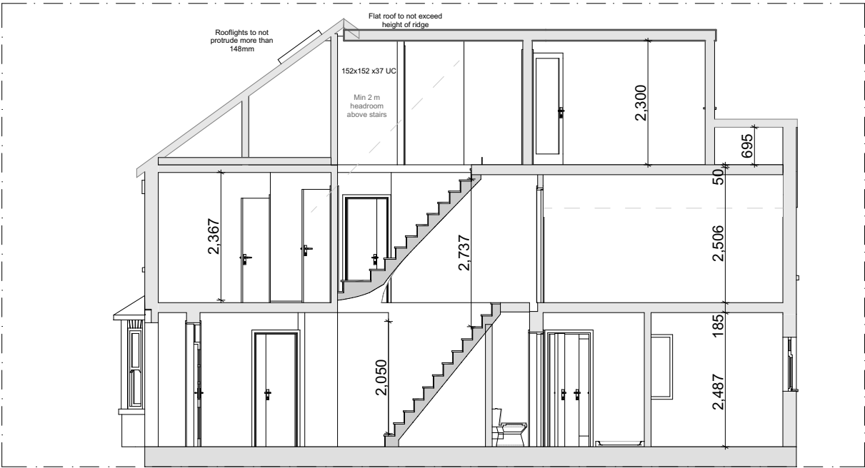
AA'5 Building Section 1:100
