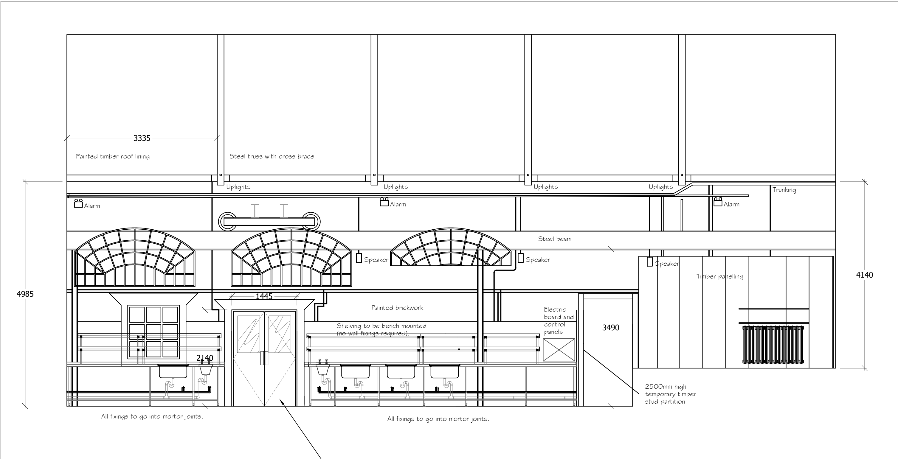
02 Section AA 02 SCALE - 1:50 @ A1
