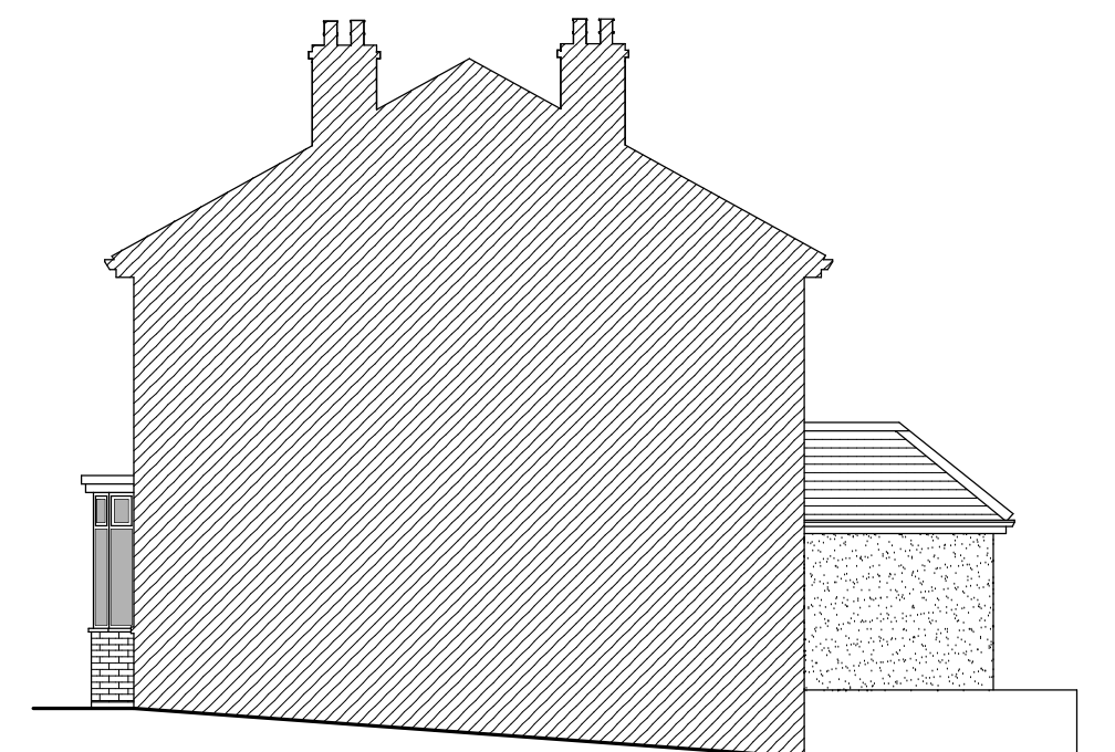
Existing Right Elevation
