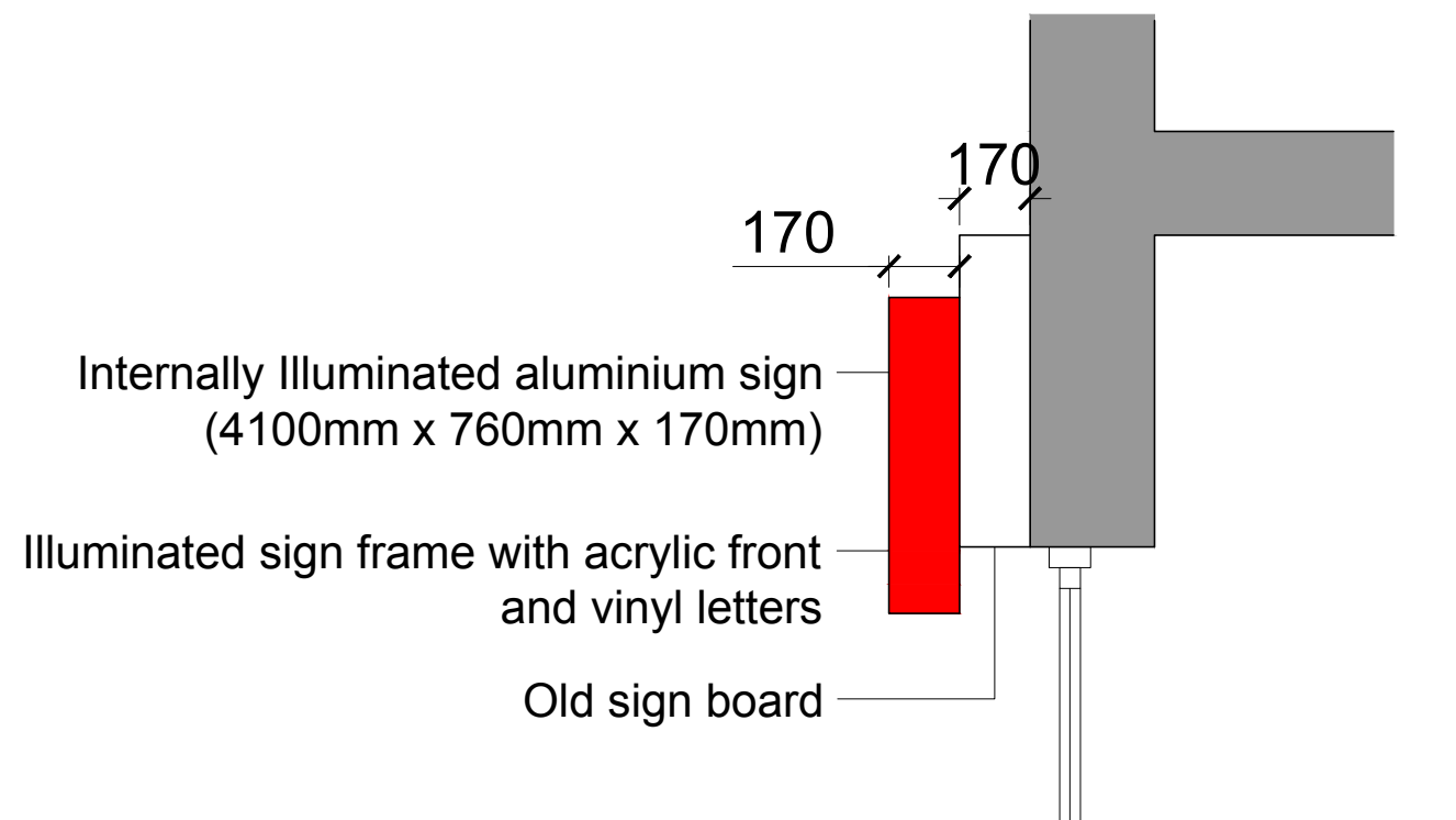
Section through Sign Scale 1:20
