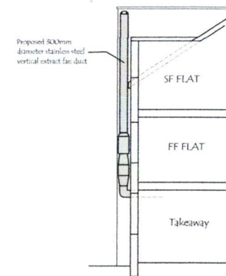
Proposed Section
