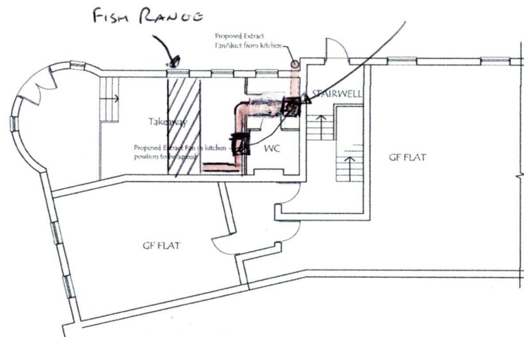
Proposed Ground Floor Plan (part)
