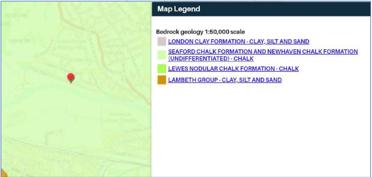
Figure 3 - Bedrock at the site. (Source: British Geological Society Website (contains British Geological Survey materials © NERC2024).
