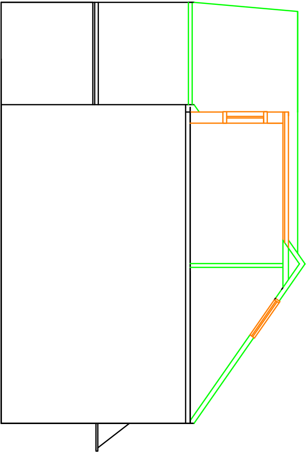
Proposed Dormer Section
