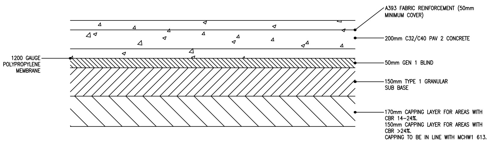
CONCRETE PAVEMENT DESIGN SCALE 1:10
