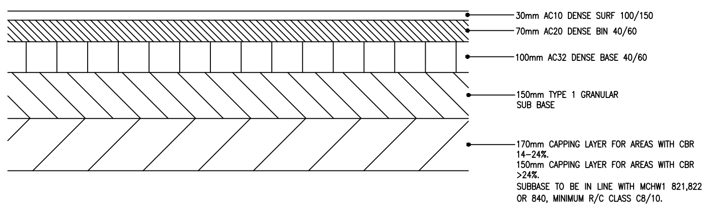
ASPHALT PAVEMENT DETAIL SCALE 1:10
