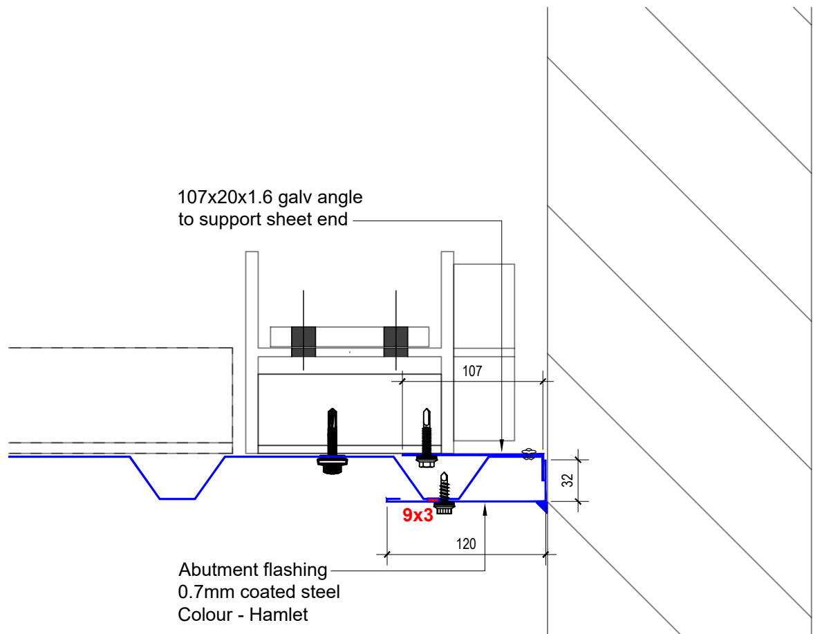
B - Wall Abutment Detail
