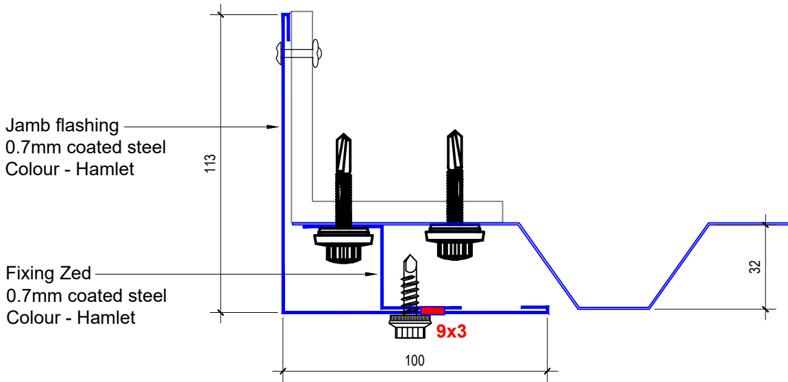
D - Opening Jamb Detail
