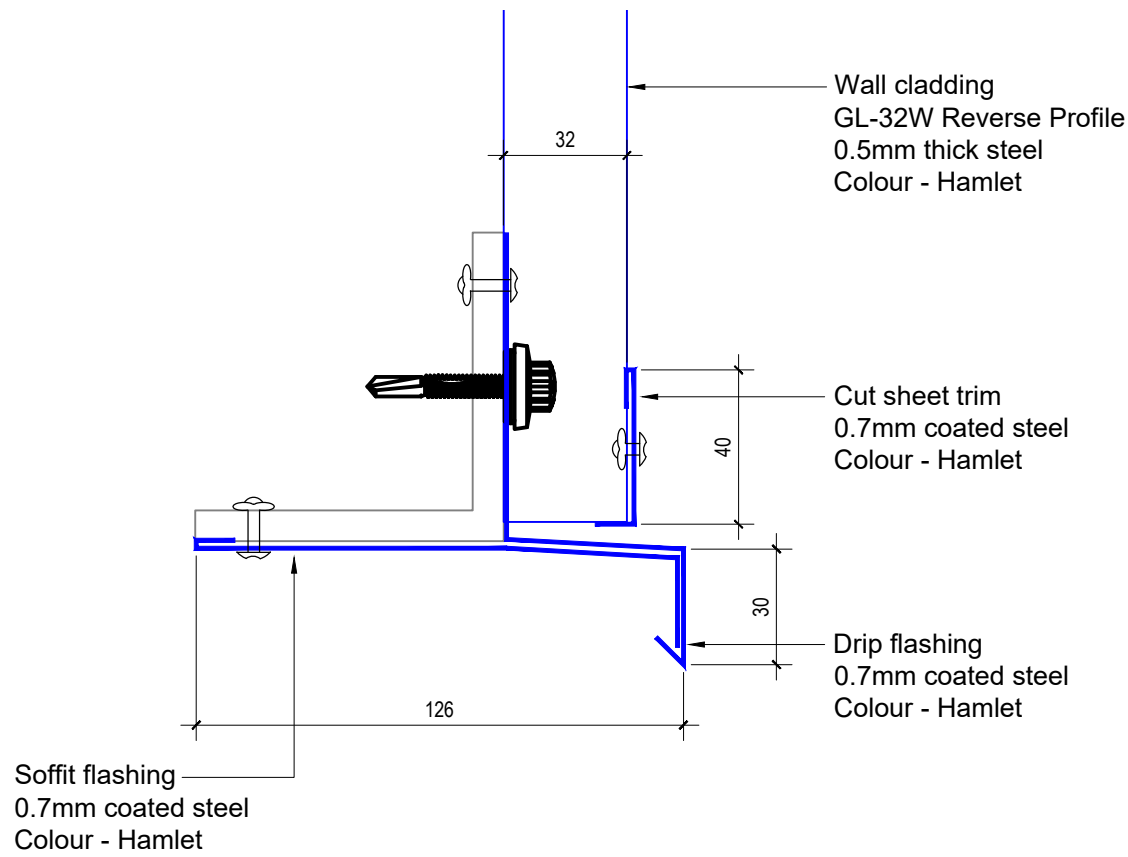
C - Opening Head Detail
