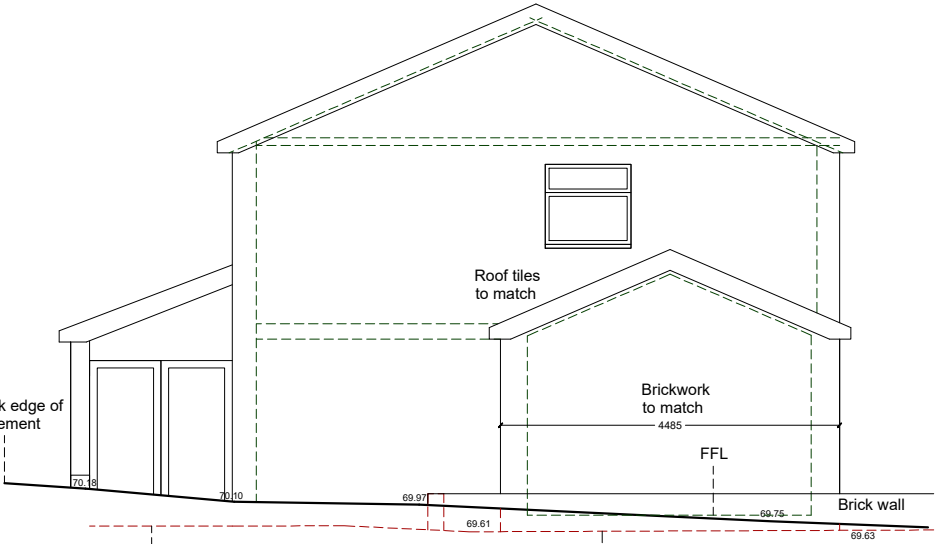
Side elevation
