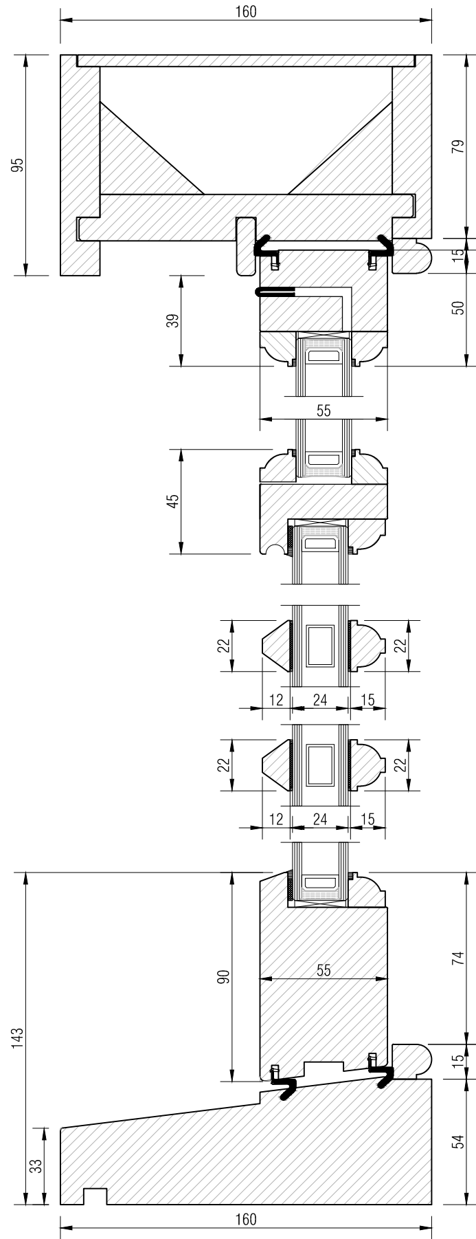
W5 SECTION SECOND FLOOR BOW WINDOW SCALE 1:2
