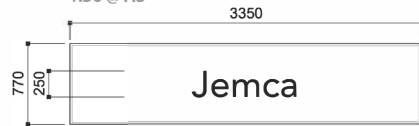
A 2No. 3350x770 Dealername Fascias - SMALL
