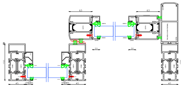
<<<<FULL WIDTH CUT THROUGH - CUT B>>>>
