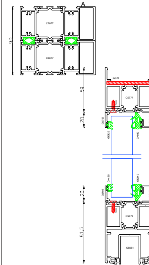
<<<<FULL HEIGHT CUT THROUGH - CUT A>>>>
