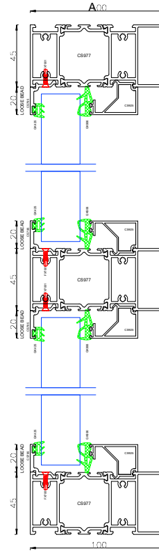
<<<<FULL HEIGHT CUT THROUGH - CUT A>>>>
