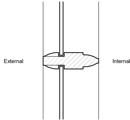
3 Window bar profile 1 : 2
