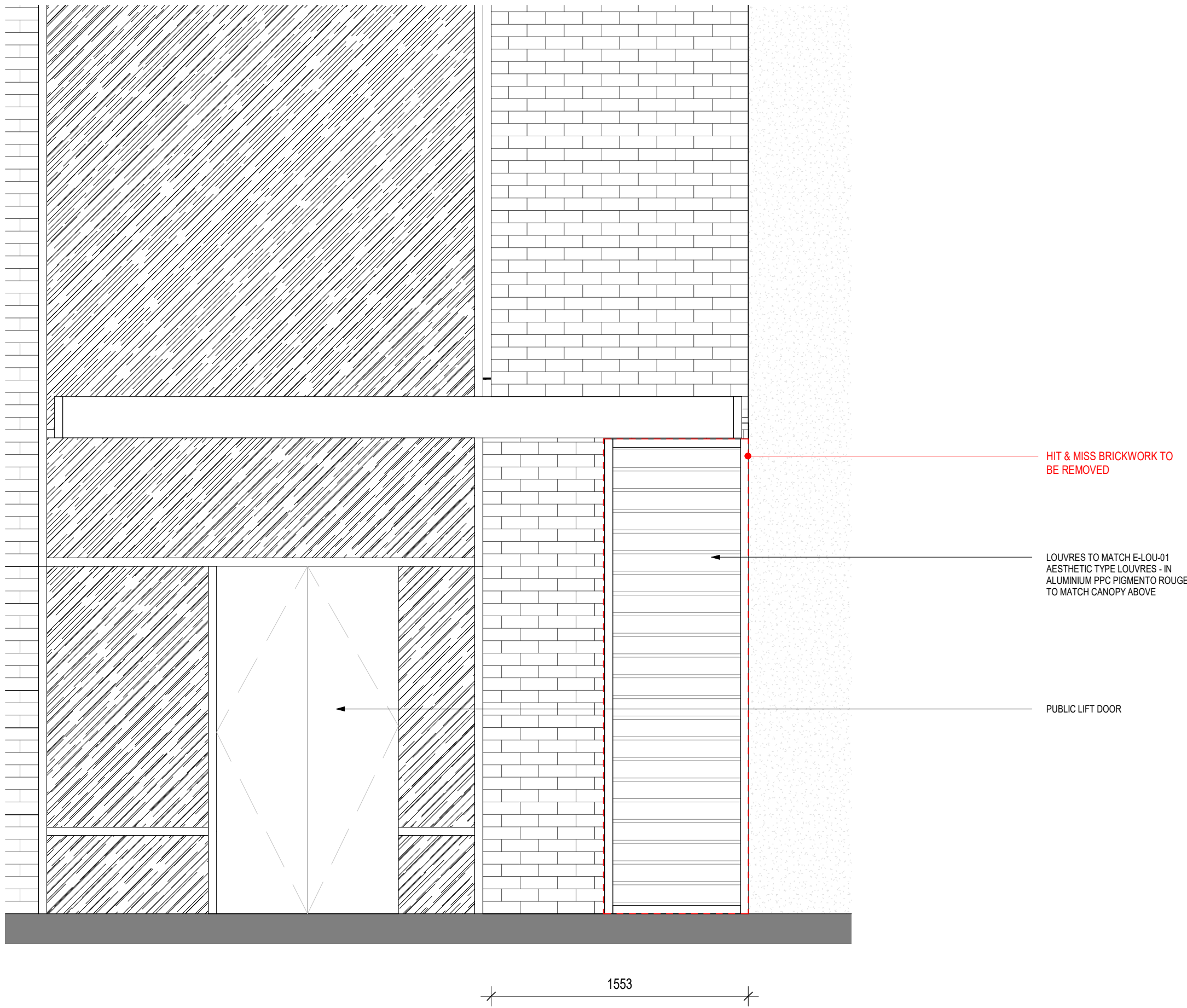
1 GARRARD STREET GAS INTAKE ELEVATION - LOUVRES
