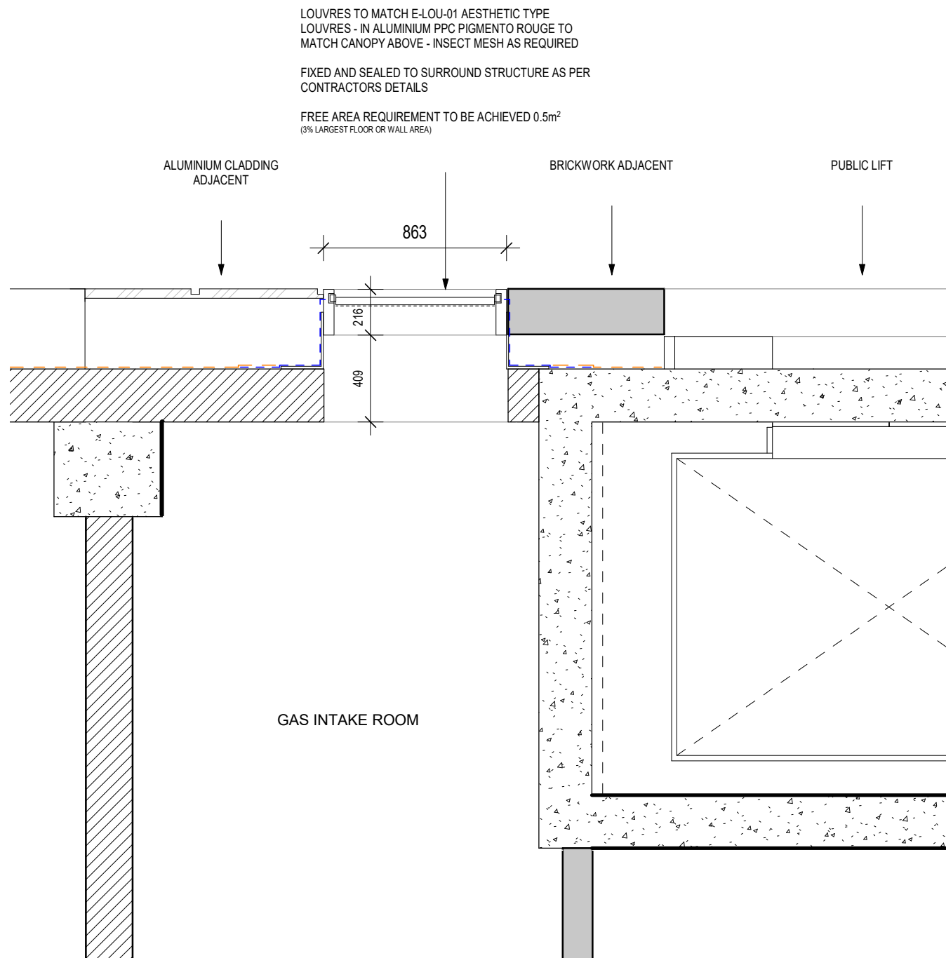
2 GARRARD STREET GAS INTAKE DETAIL PLAN - LOUVRES
