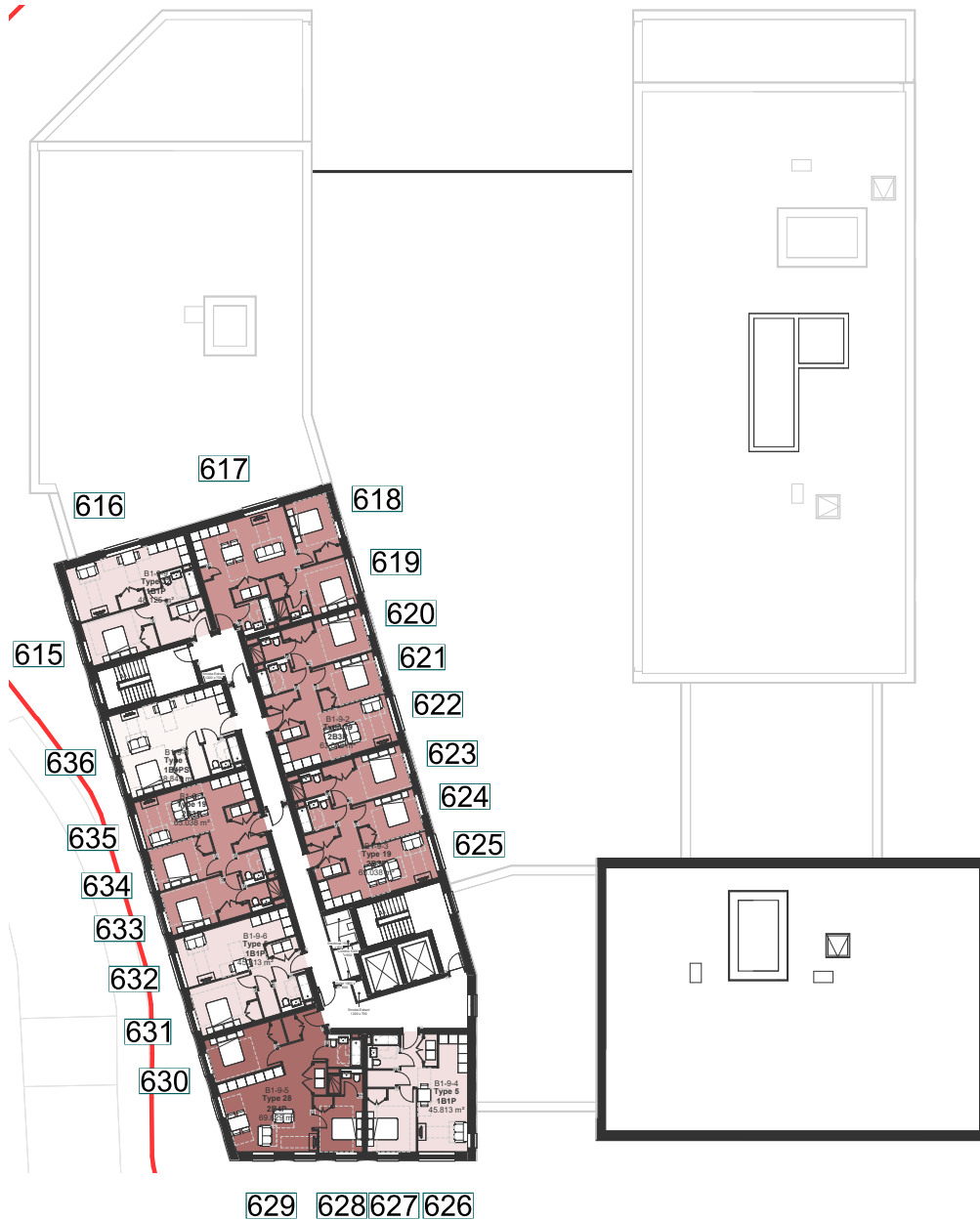
Fig. 20: Floor Plan
