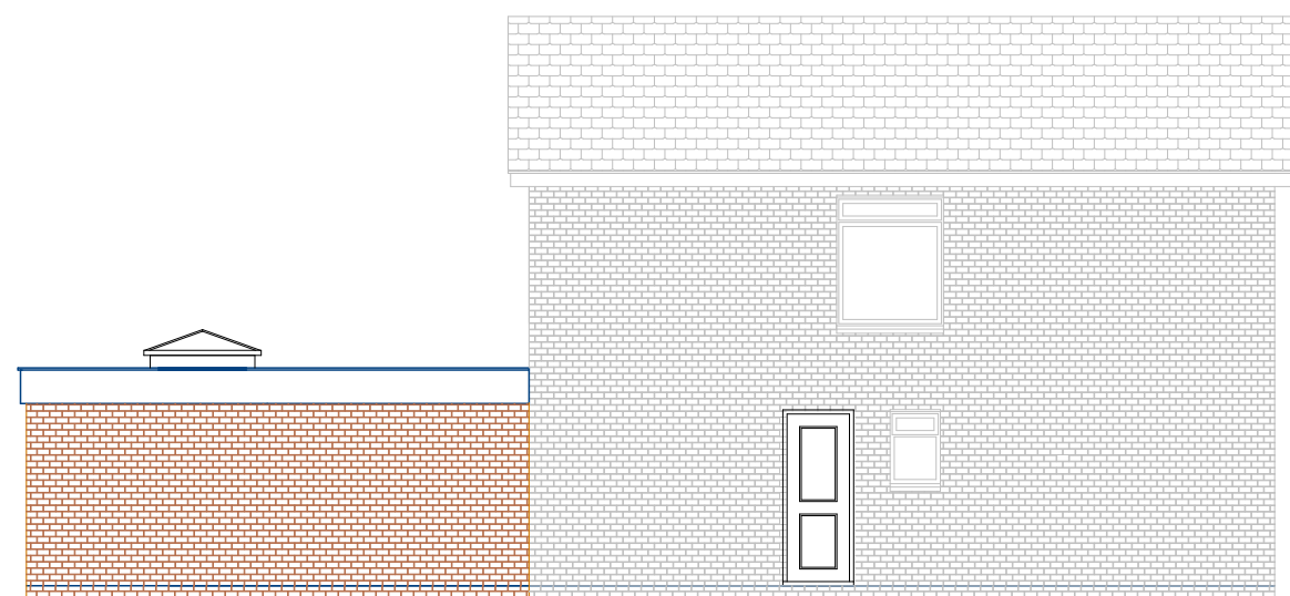
Proposed Side Elevation (L)
