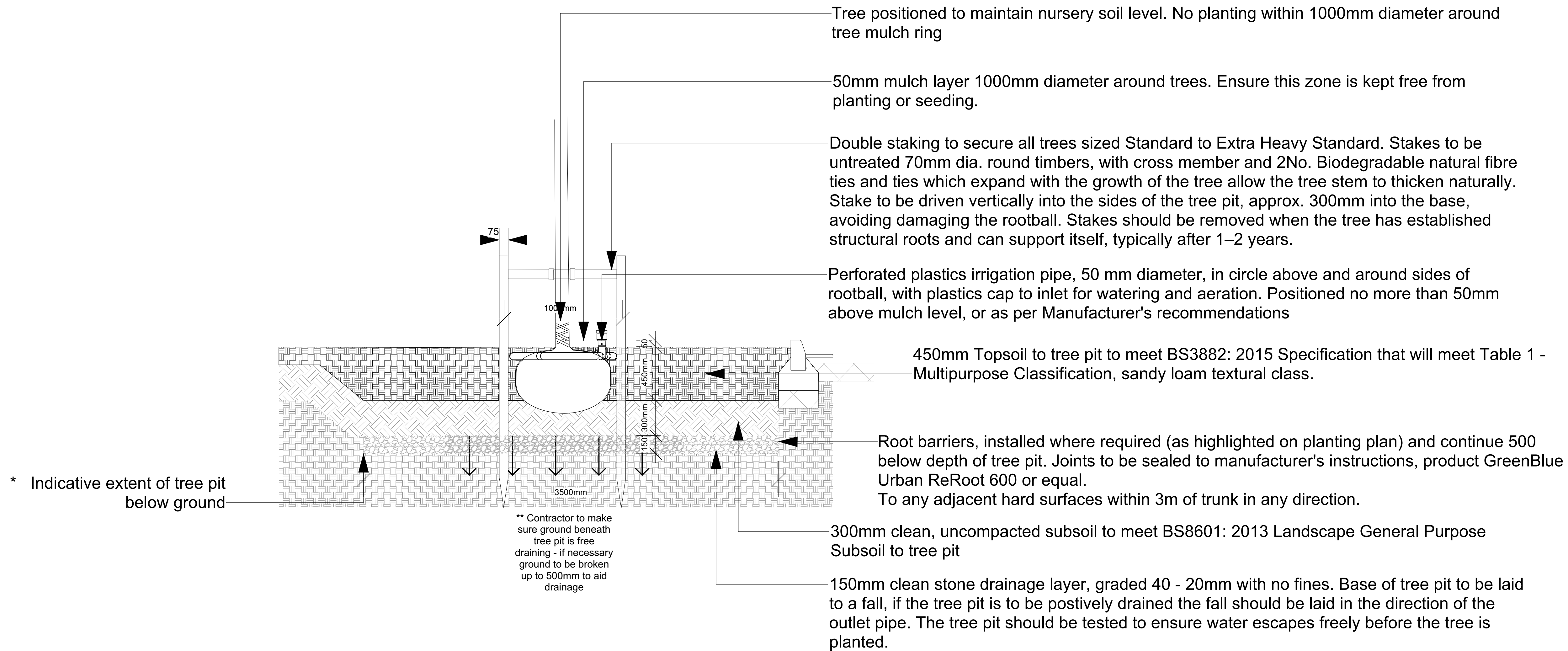
1 Tree Pit in Soft Scale: 1:20
