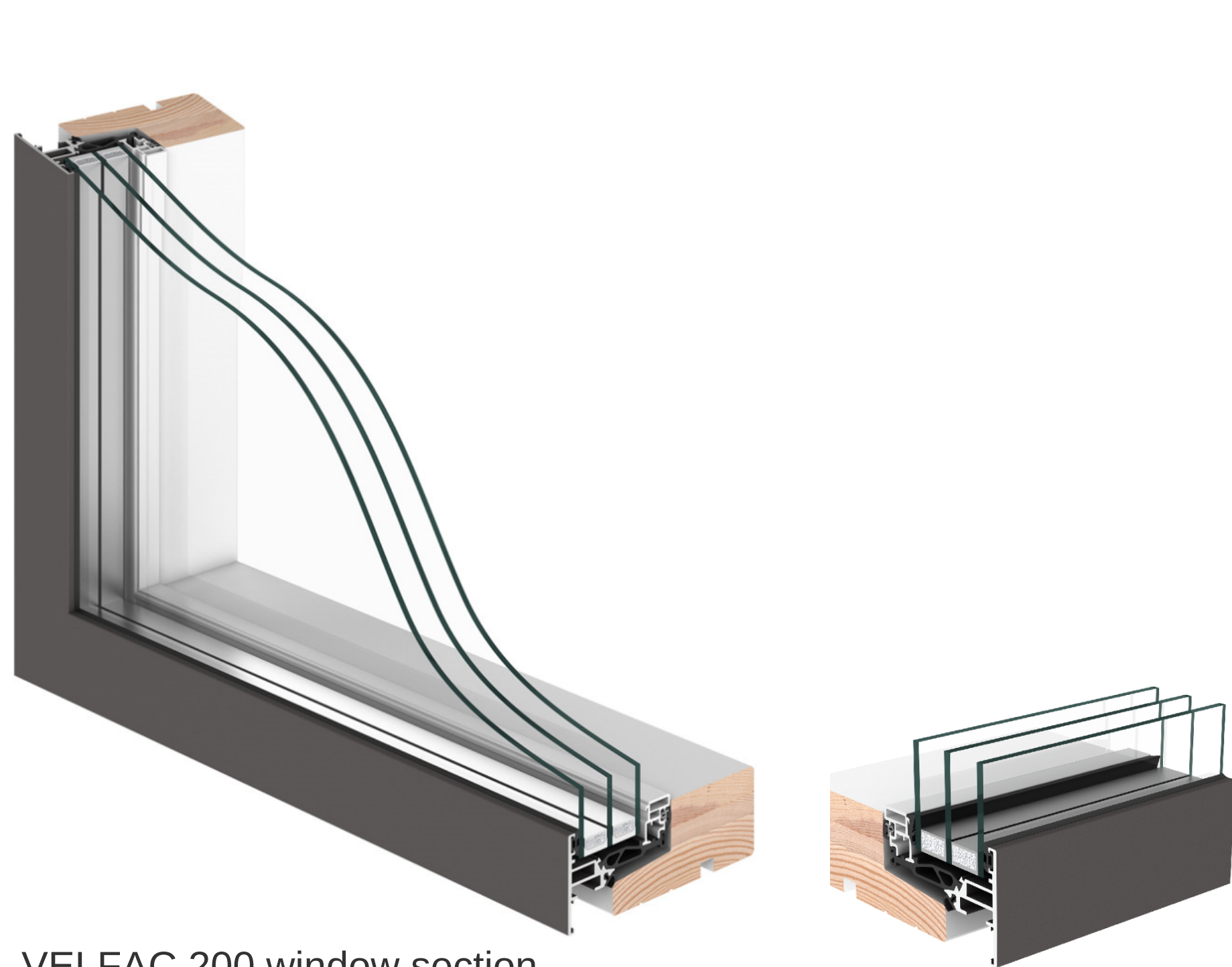
VELFAC 200 window section
