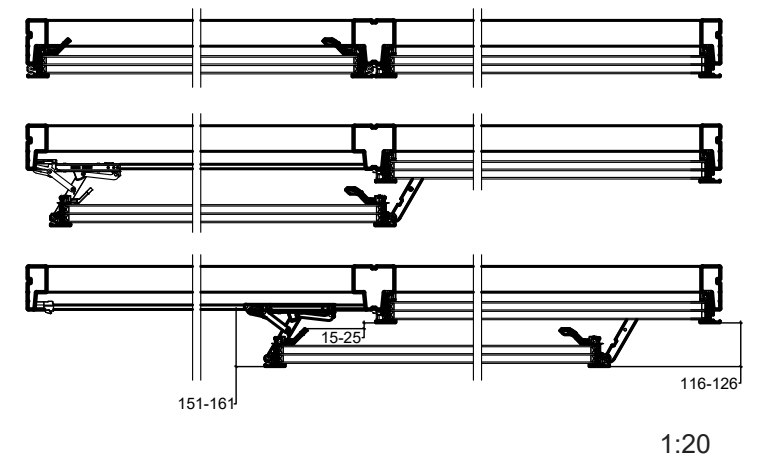
VELFAC 200 ENERGY, sliding casement door, 70mm threshold
