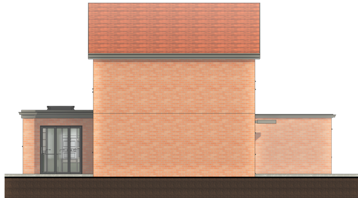
2 East Coloured 1 : 100
