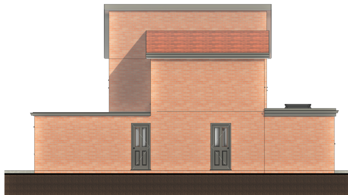
4 West Coloured 1 : 100
