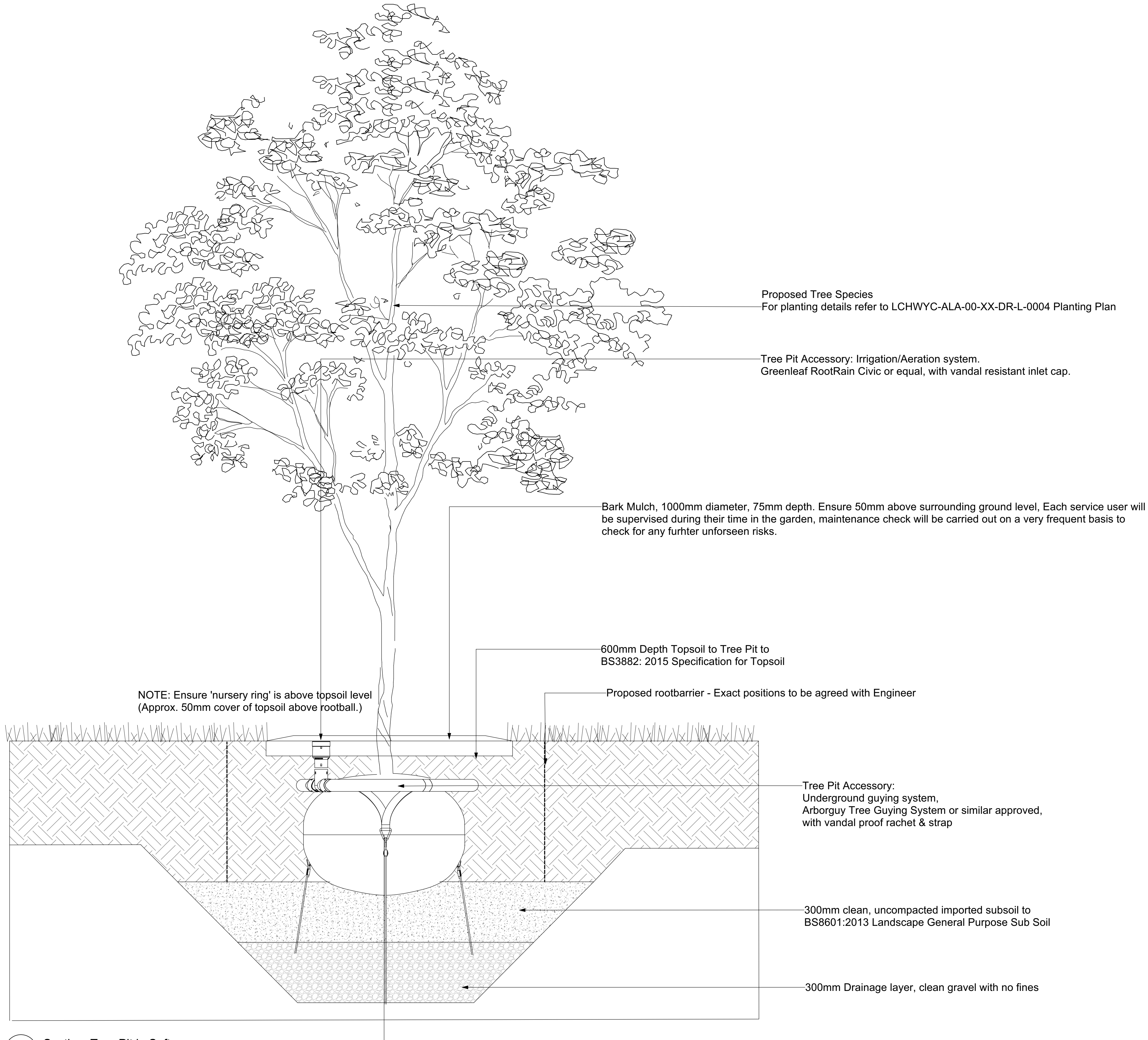
1 Section: Tree Pit in Soft Scale: 1:10
