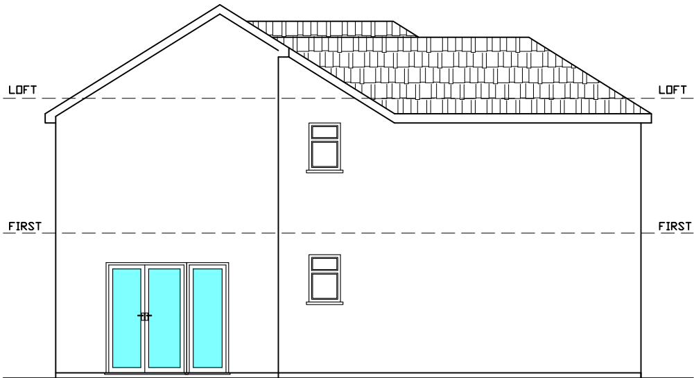
PROPOSED LEFT SIDE ELEVATION
