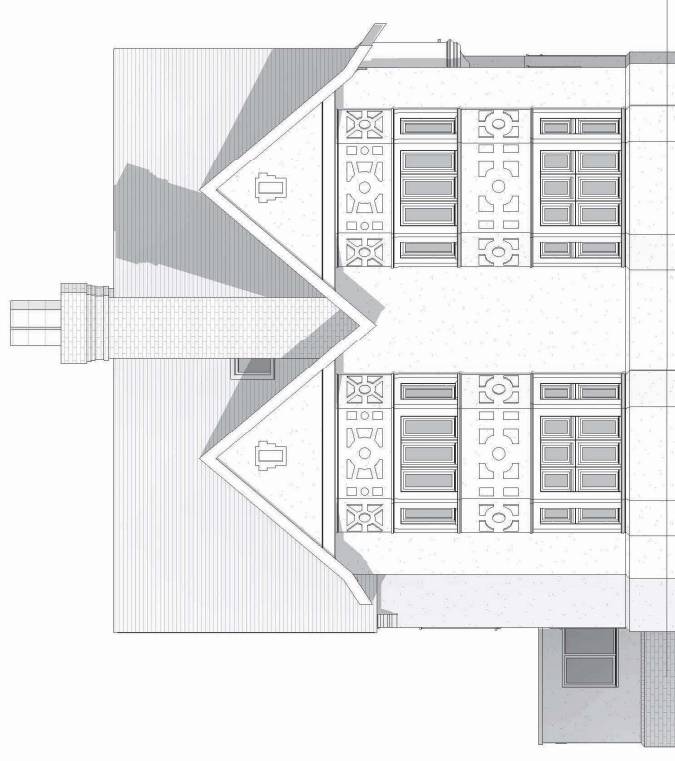
Side 2 Elevation
