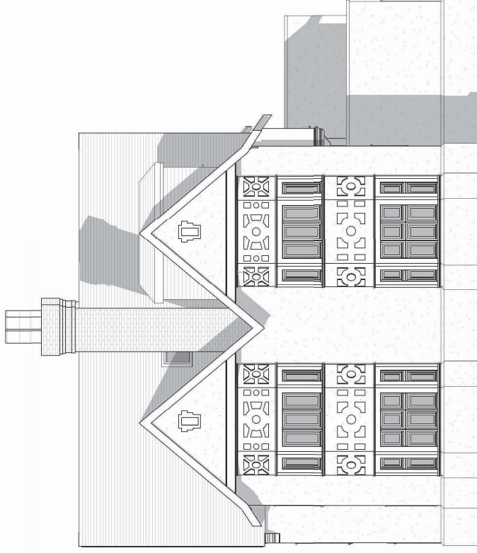
Side 2 Elevation
