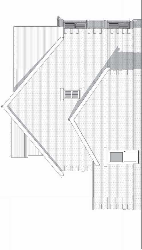
Side 1 Elevation
