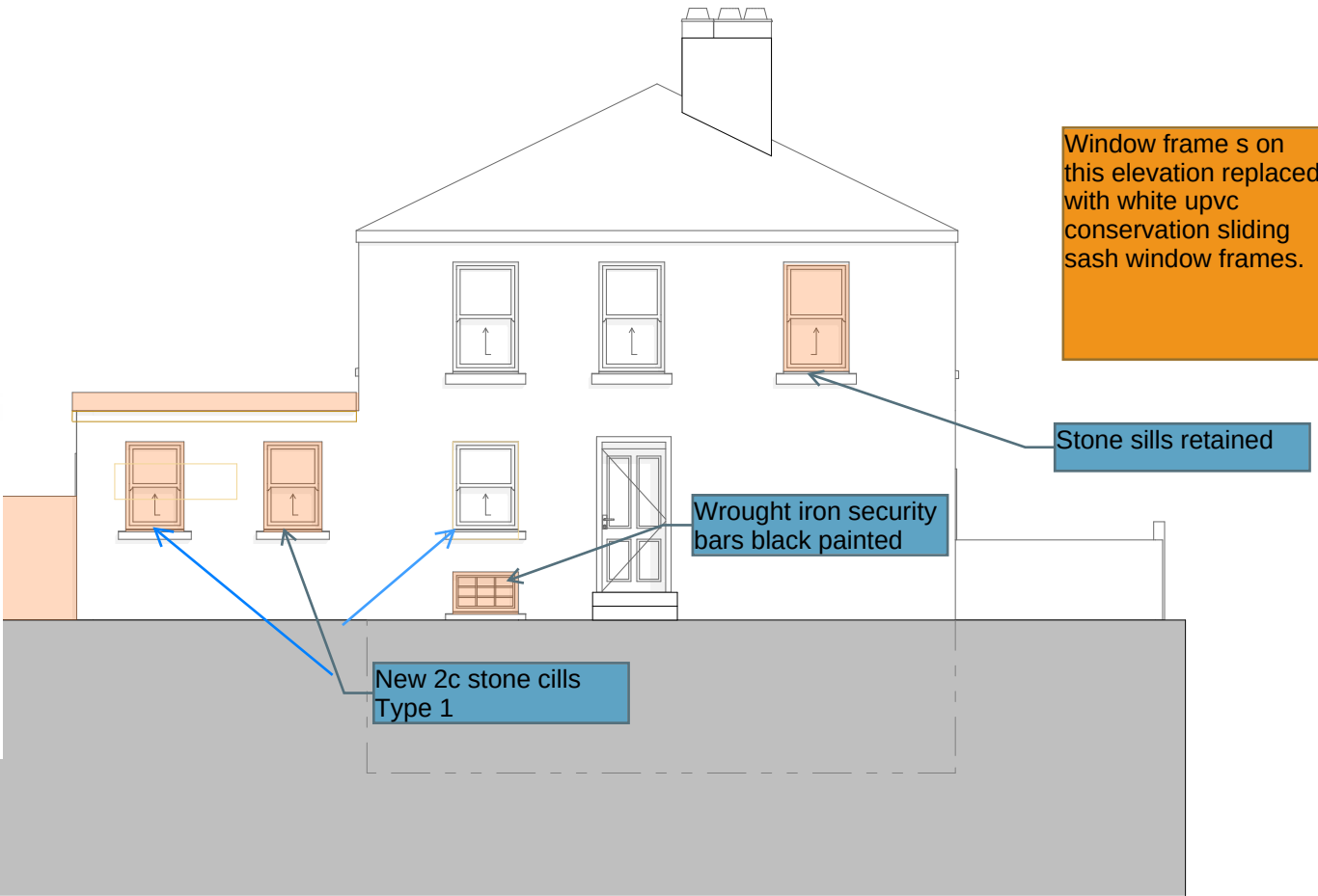
1:100 Proposed Left Side Elevation
