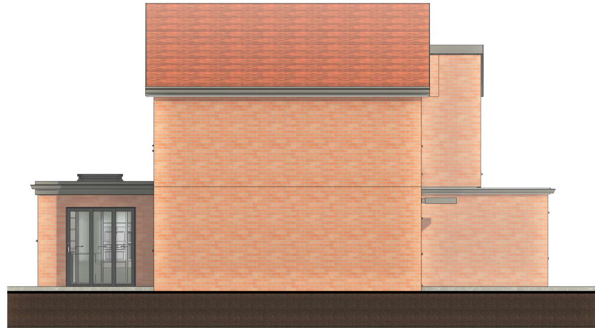
2 North. Coloured 1 : 100
