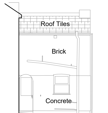
Existing East Elevation 1 : 100
