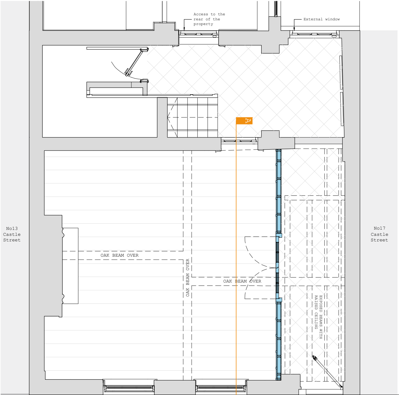
N AS PROPOSED GROUND FLOOR PLAN - 1:50 @ A3 (FRONT CELL) SHOWING THE LOCATION OF NEW PARTITION IN BLUE
