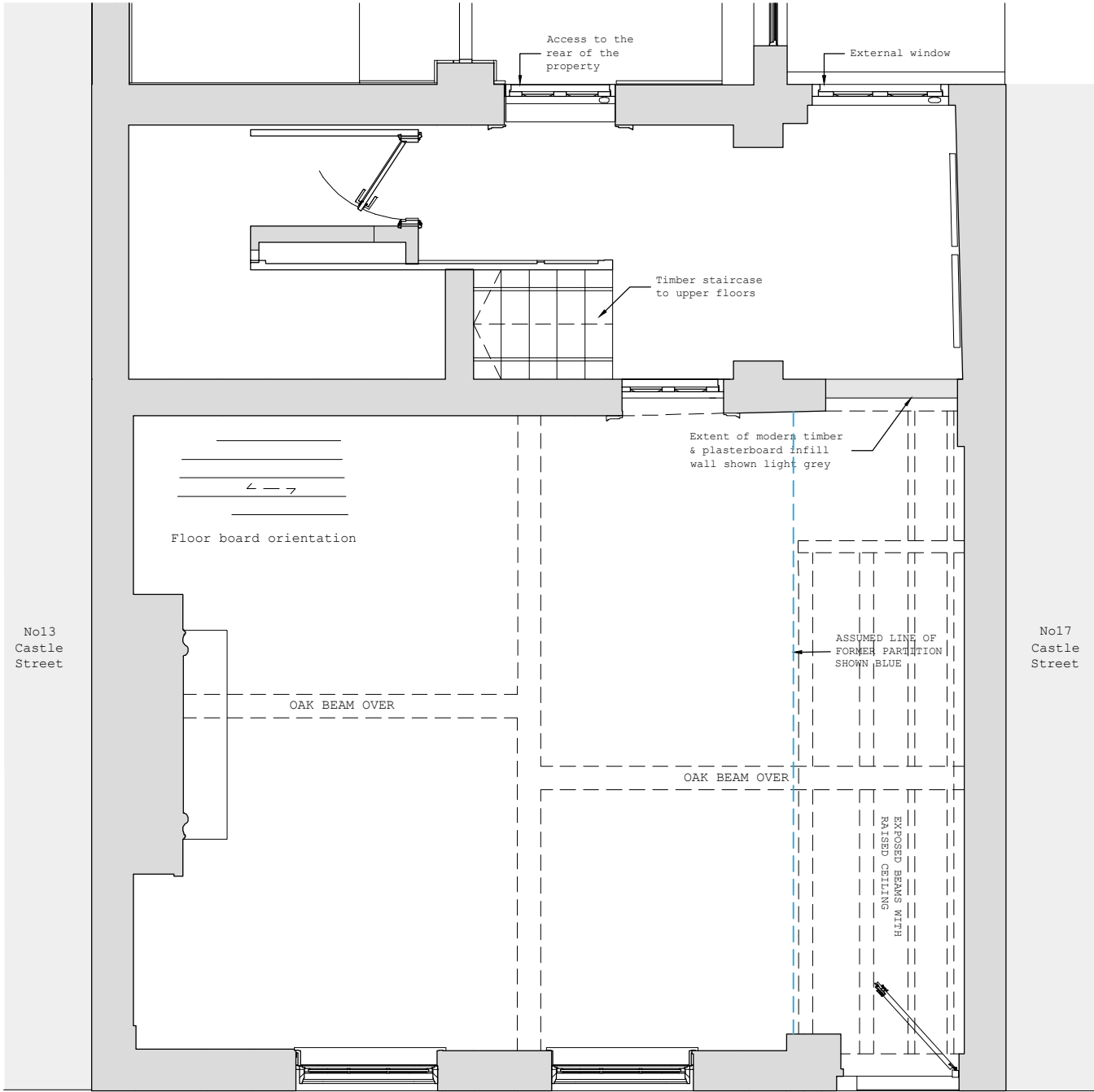
N AS EXISTING GROUND FLOOR PLAN - 1:50 @ A3 (FRONT CELL). ASSUMED LINE OF FORMER PARTITION SHOWN BLUE DOTTED
