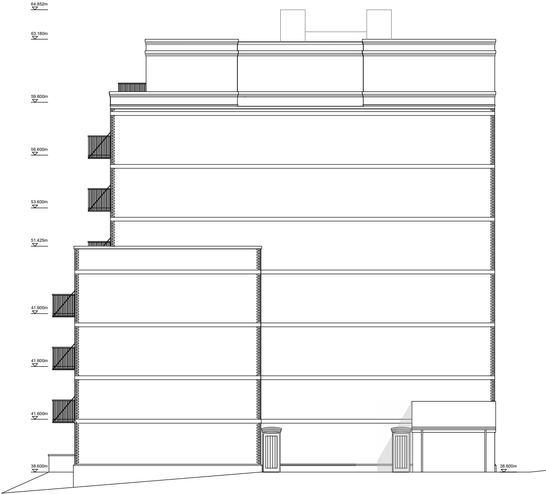
Northwest Elevation 3-3
