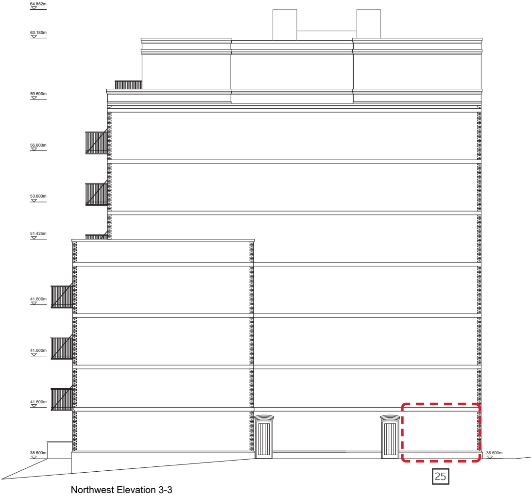
Northwest Elevation 3-3
