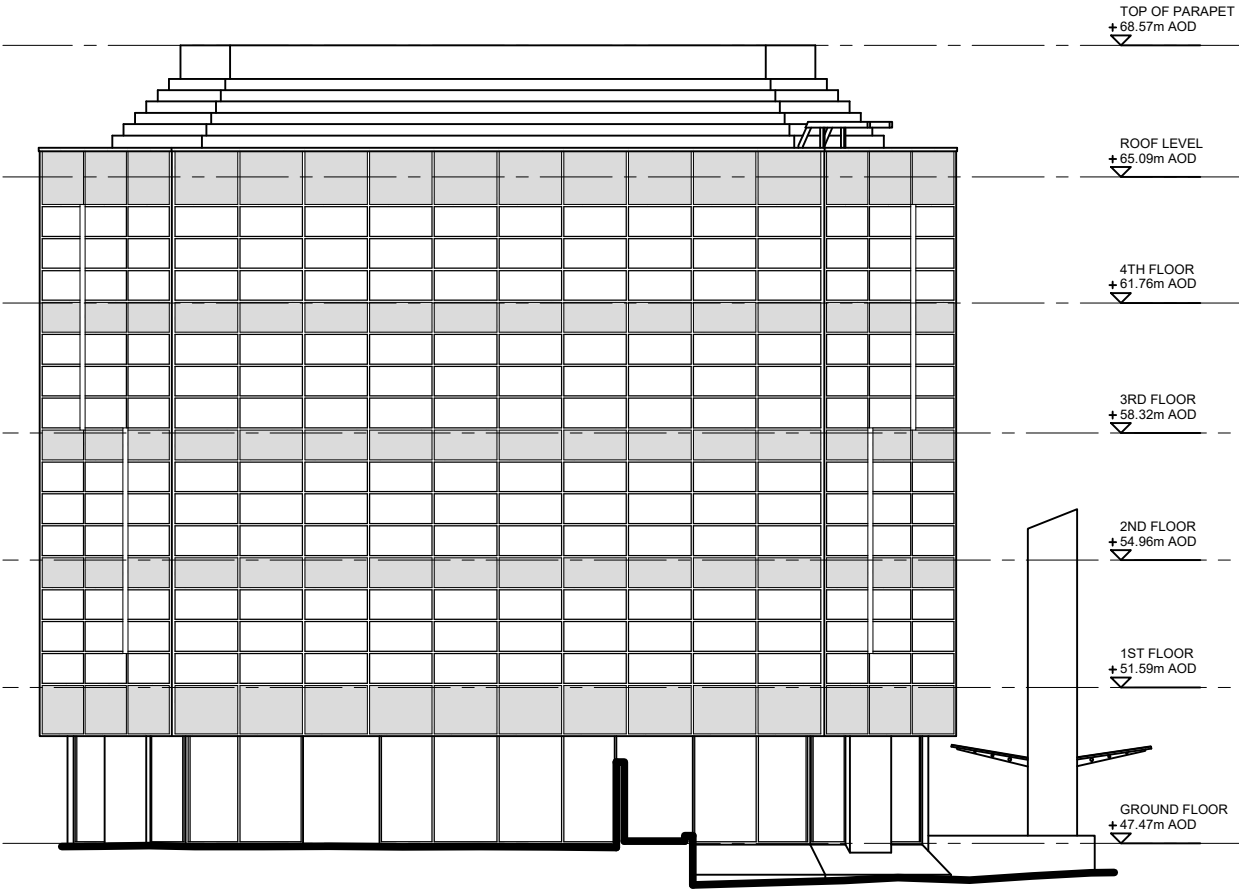
EAST ELEVATION
