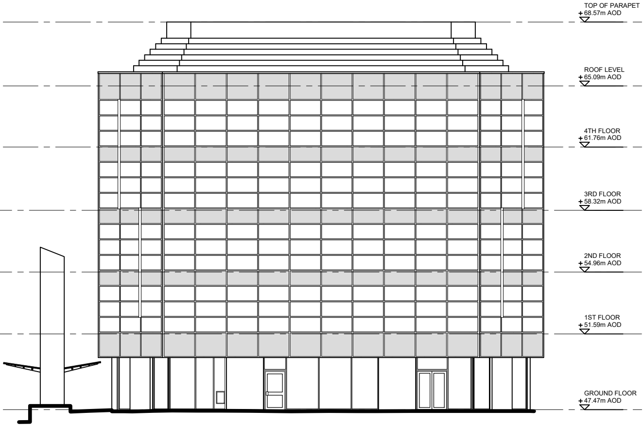
WEST ELEVATION
