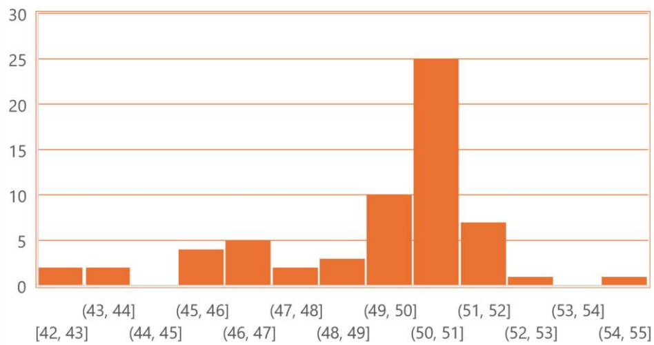
LA90 Histogram 07:00 - 23:00
