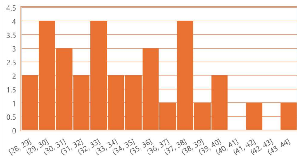
LA90 Histogram 23:00 - 07:00
