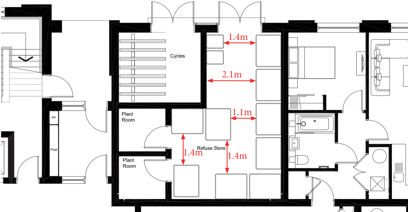
Proposed Refuse store in Railway House (Block A).
