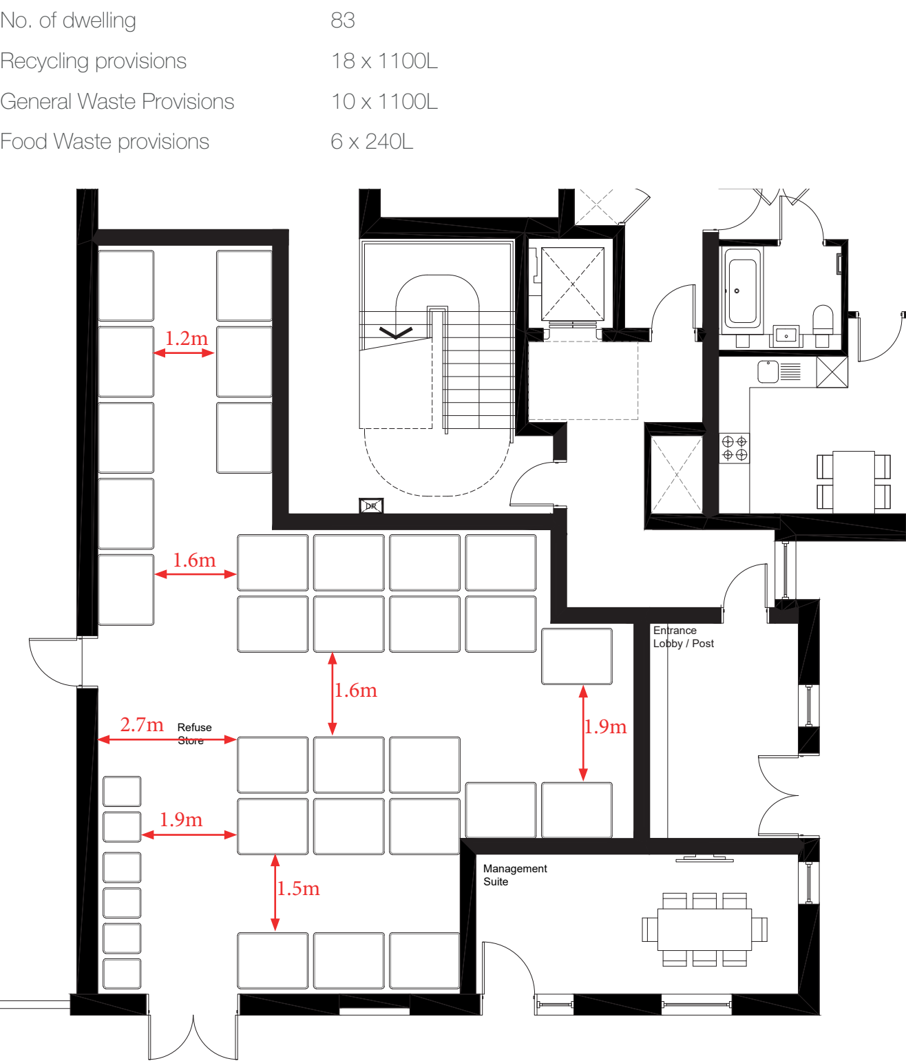
Proposed Refuse store in Goods Warehouse (Block B).
