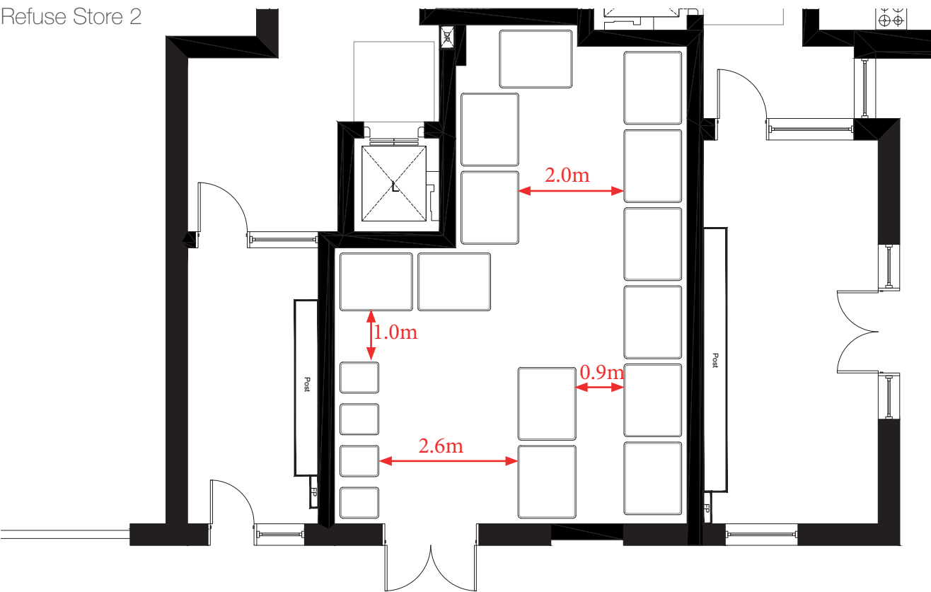
Approved Refuse store in Goods Warehouse (Block B).
