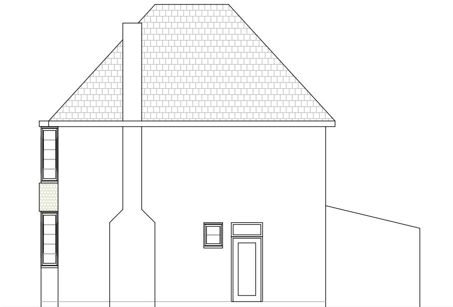
Existing Alternate Side Elevation
