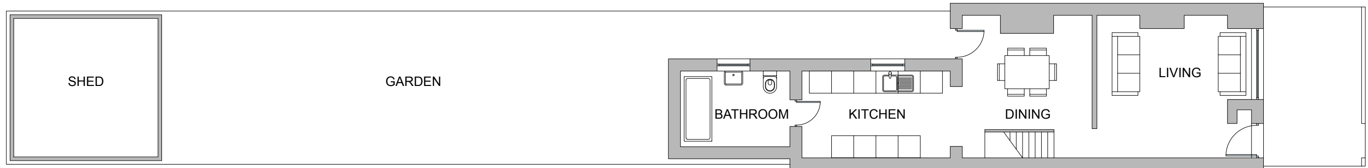
GROUND FLOOR
