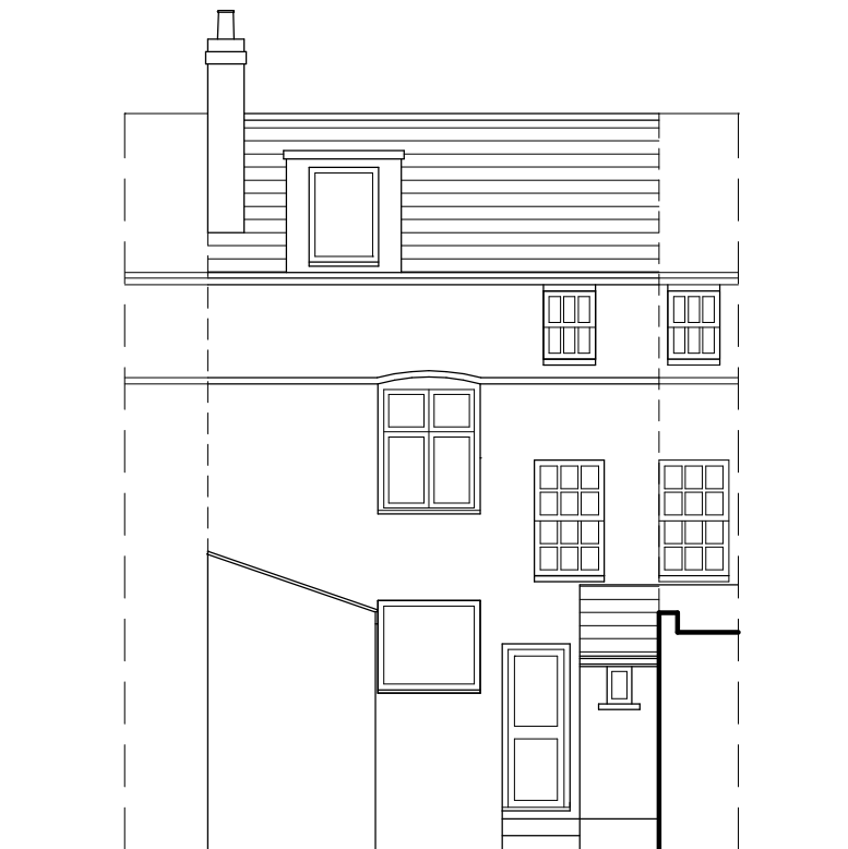
REAR ELEVATION
