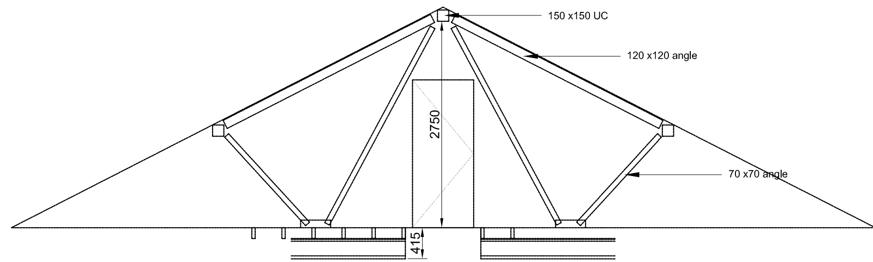
14038_013 EXIST LR / 01 ST GILES HOUSE - EXISTING ROOF SECTION scale 1:50
