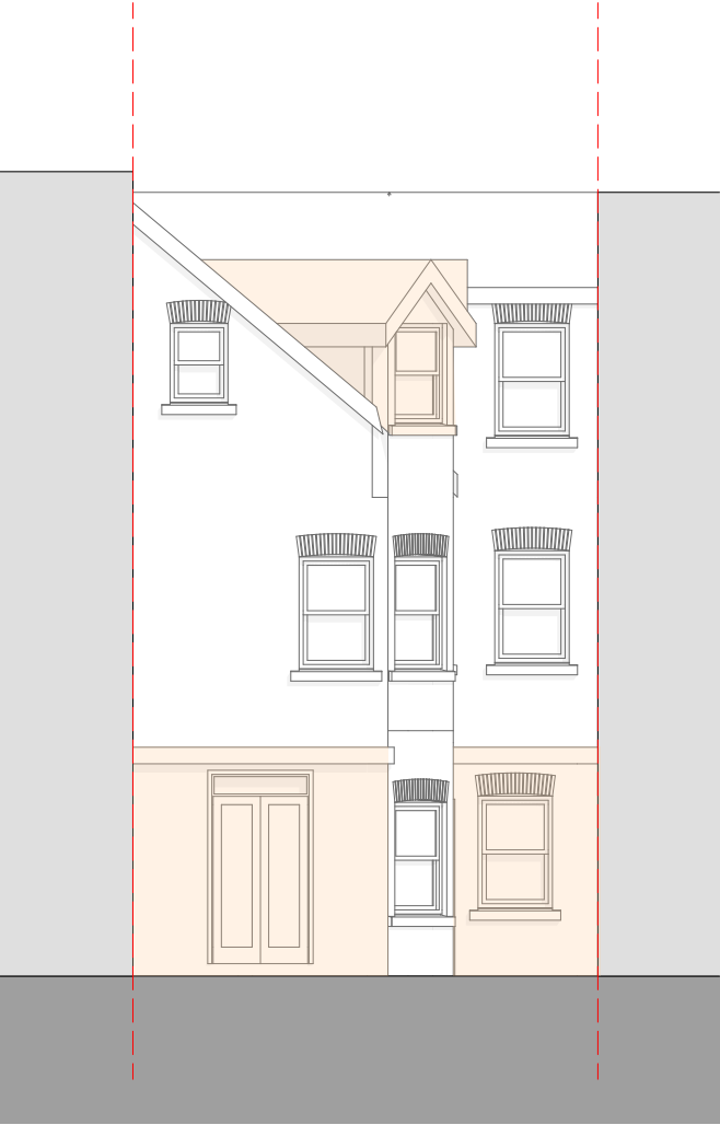
1:100 Rear Elevation
