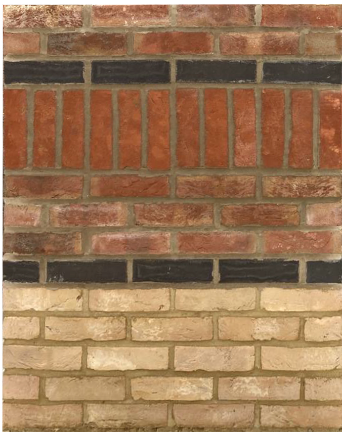
Panel 1 Photograph of a built sample panel
