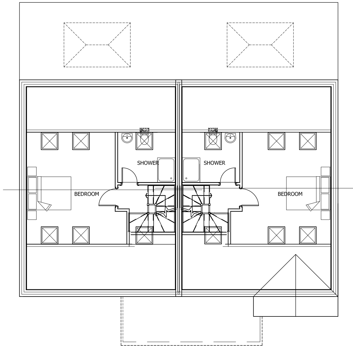
Loft Floor Plan ( Bedroom and bathroom) 34.25m 2
