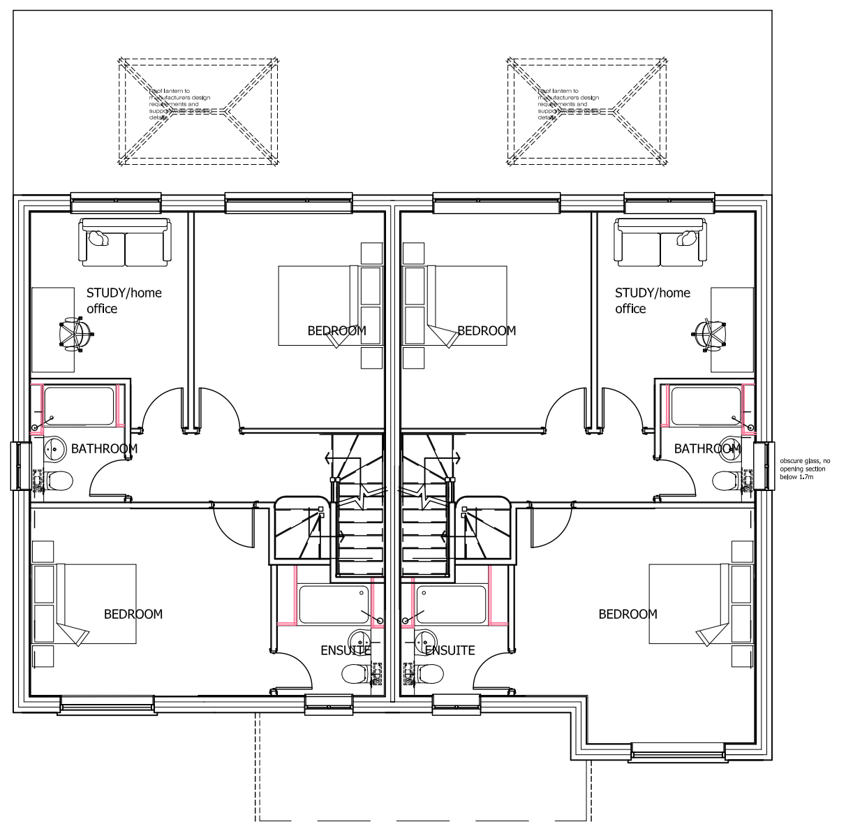
First Floor Plan (2bedrooms, Study, 2 baths) 65.0m 2
