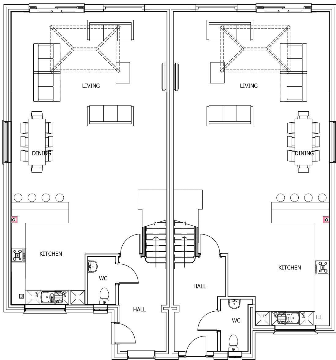
Ground Floor Plan 88.6m 2
