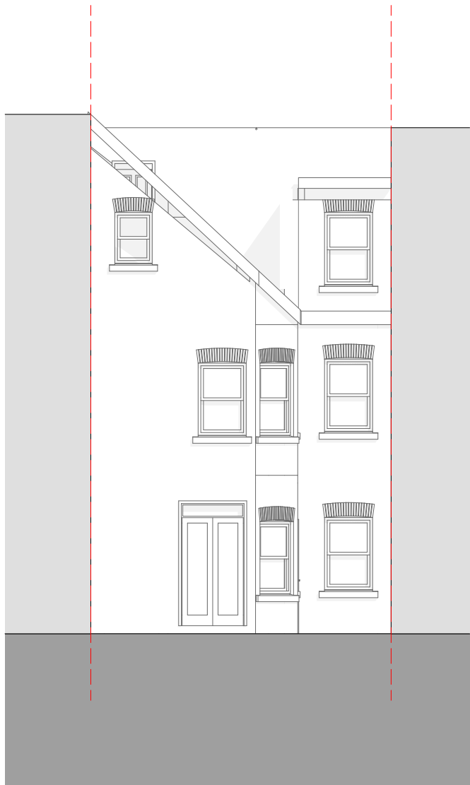
1:100 Rear Elevation
